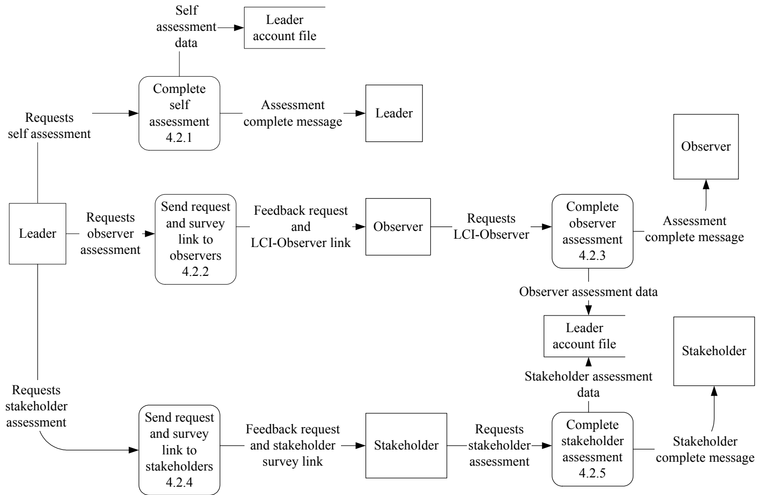
Figure 16. Level 2 DFD for process 4.2 (Add to existing assessment).
